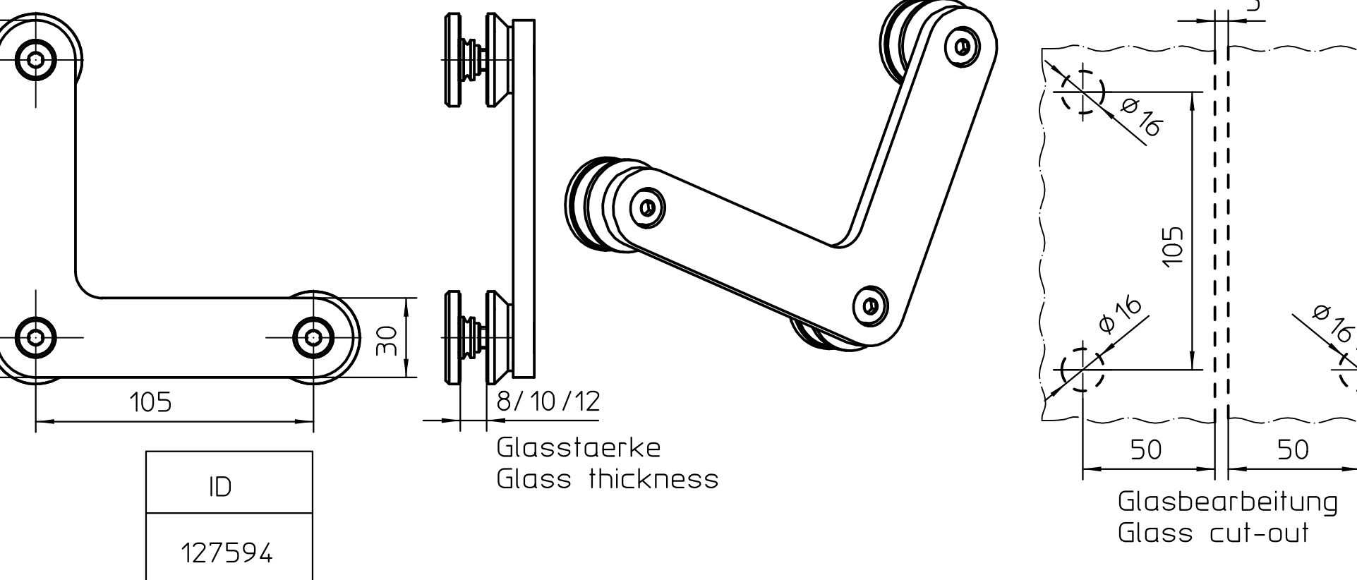
Glas - Glas Eckverbinder, einstellbar Glass - glass corner connector, adjustable
