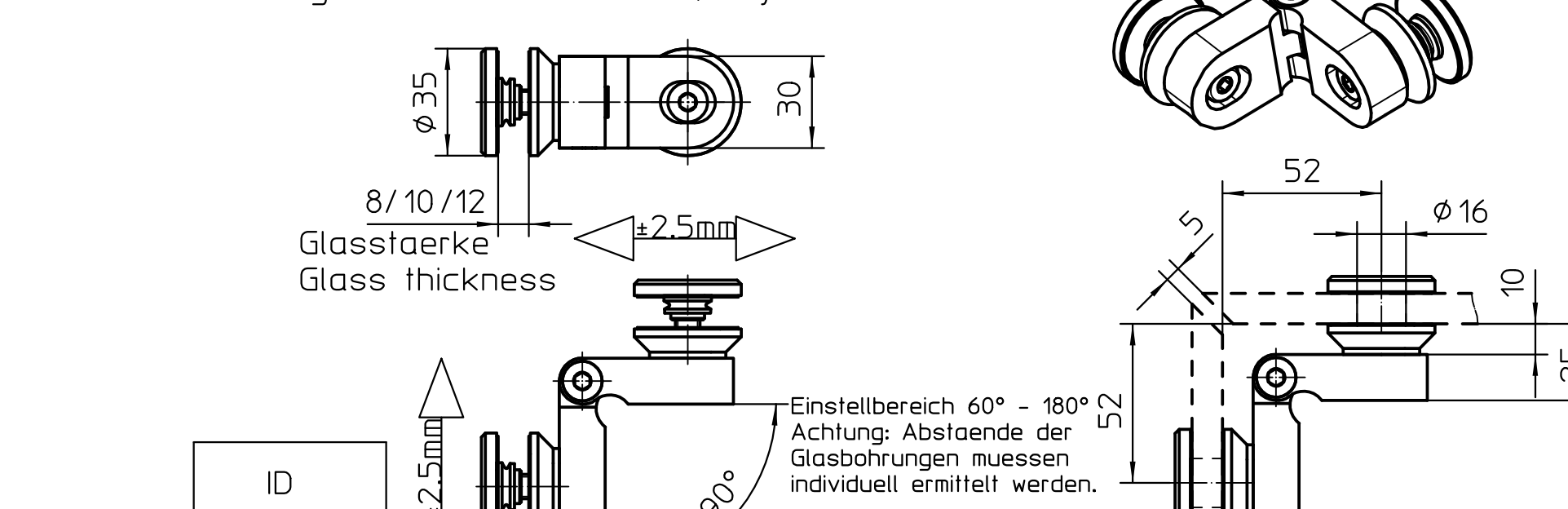
Glas - Glas Eckverbinder, einstellbar Glass - glass corner connector, adjustable
