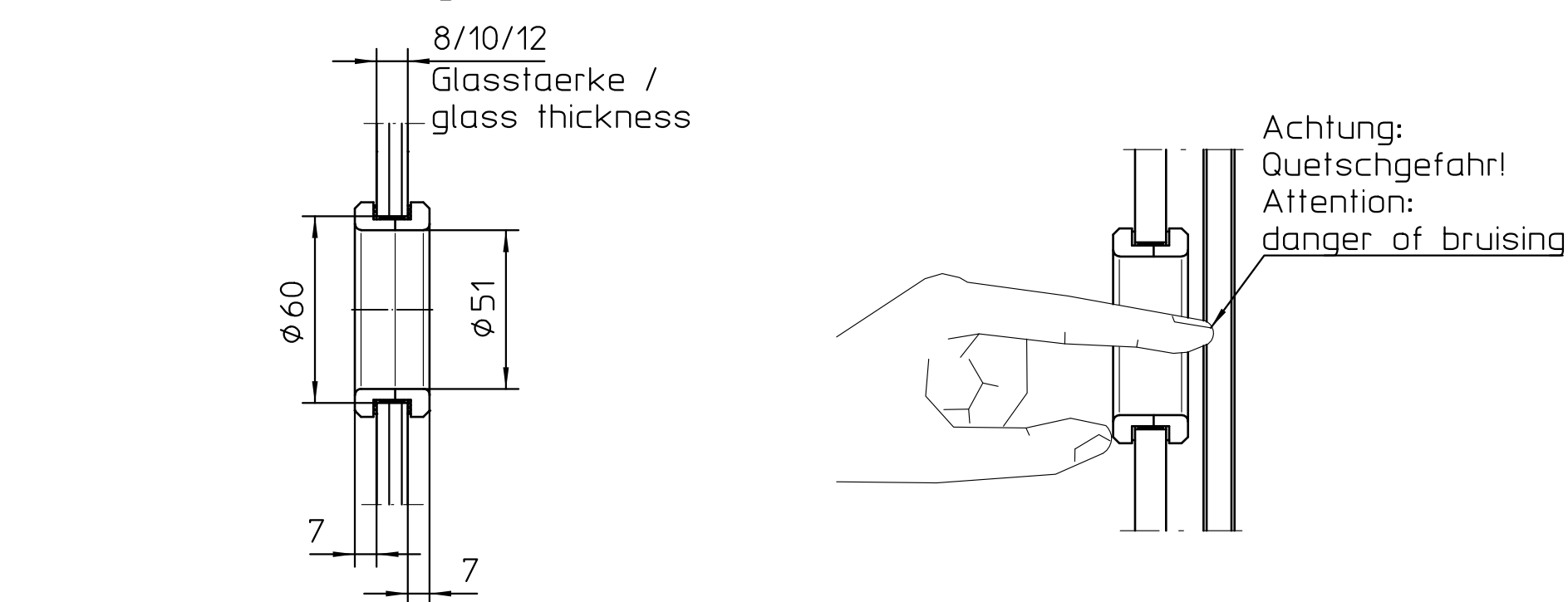
Griffmuschel 8-12mm Glas Recess knob 8-12mm glass
