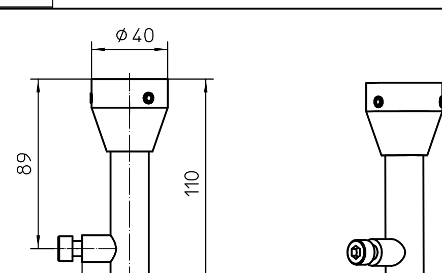
Deckenhalter verstellbar Aeralan Ceiling mount adjustable Aeralan
