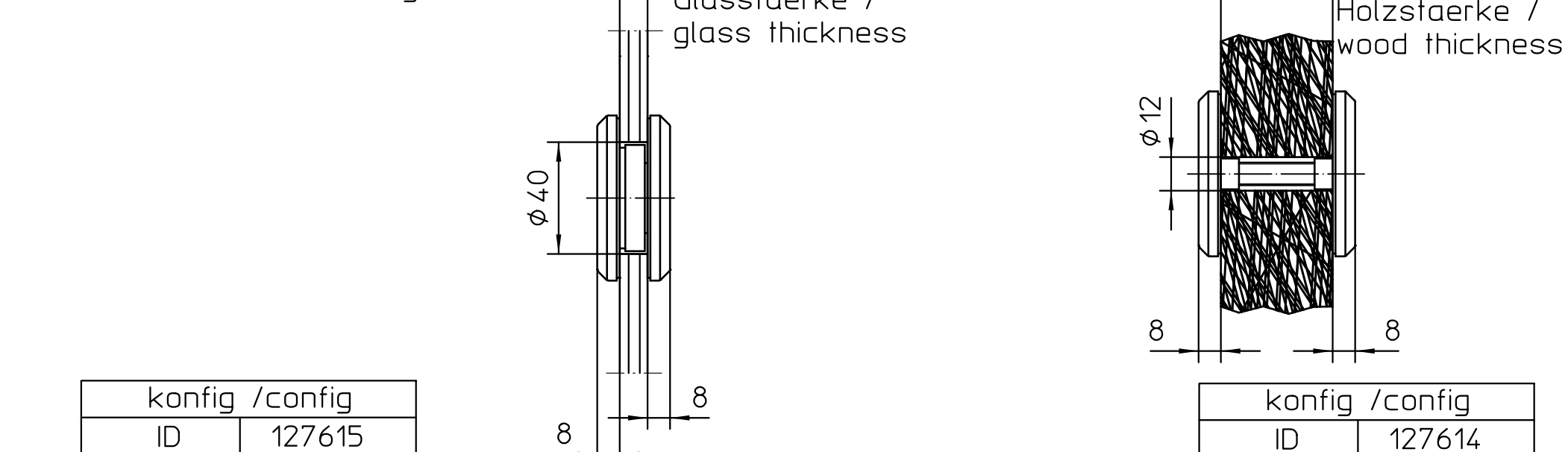
Griffmuschel 8-12mm Glas Recess knob 8-12mm glass
